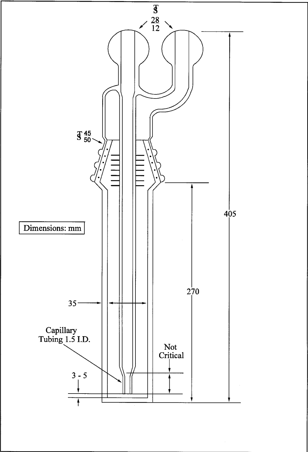
Figure 7C-2. Restricted-Orifice Impinger.
