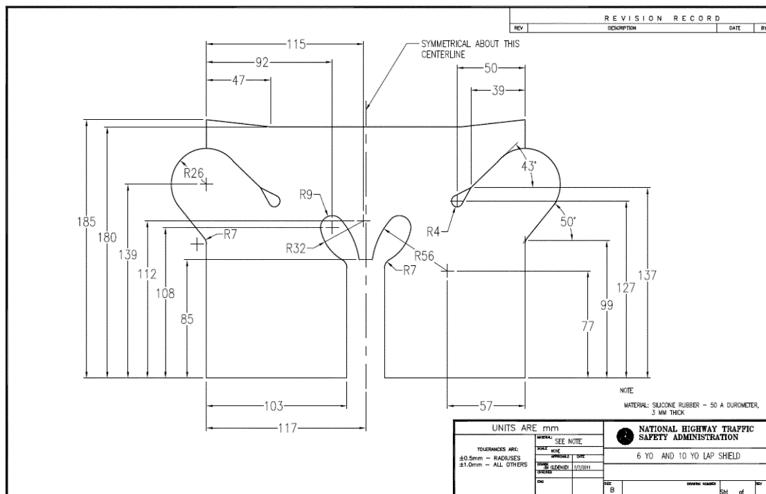
Figure 13 – Lap Shield
