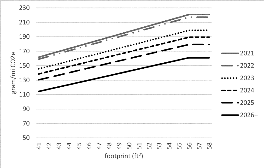
Figure 3 Car Curves
