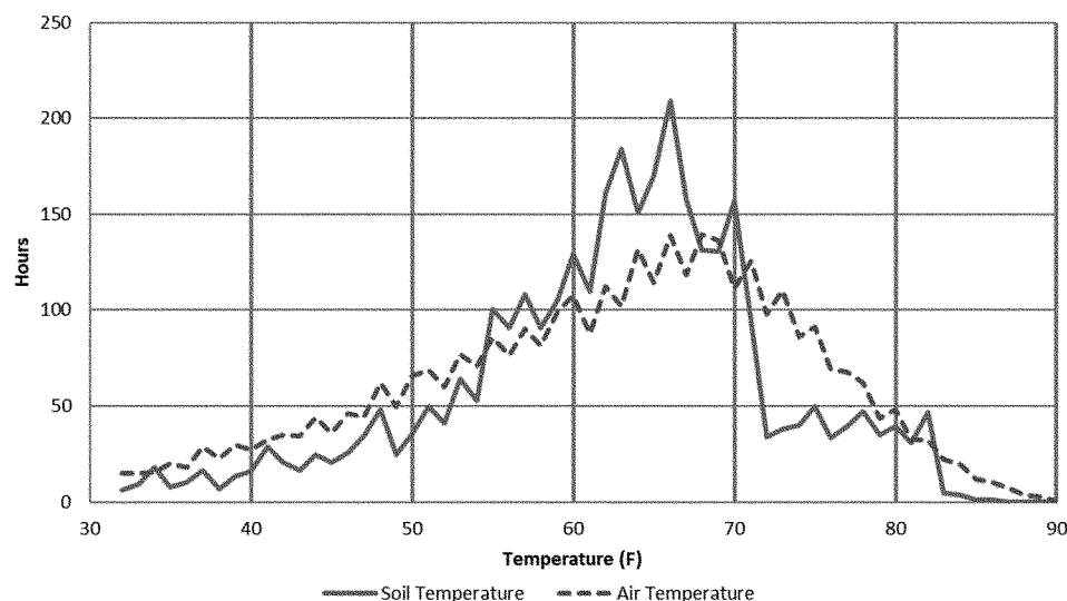
Figure 1: Weighted-Average Air and Soil Temperature during Dehumidification Season (April – October)
