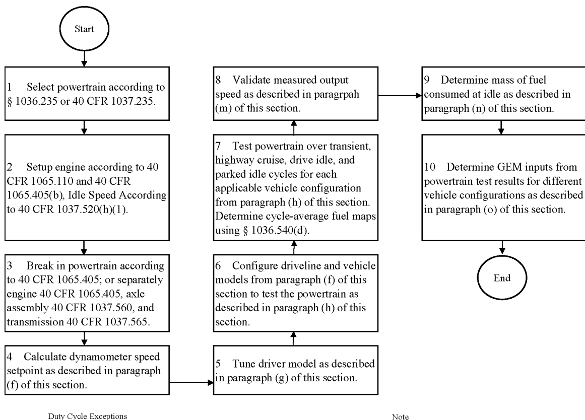
Figure 1 to Paragraph (a)(11) of § 1036.545—Overview of Powertrain Testing
