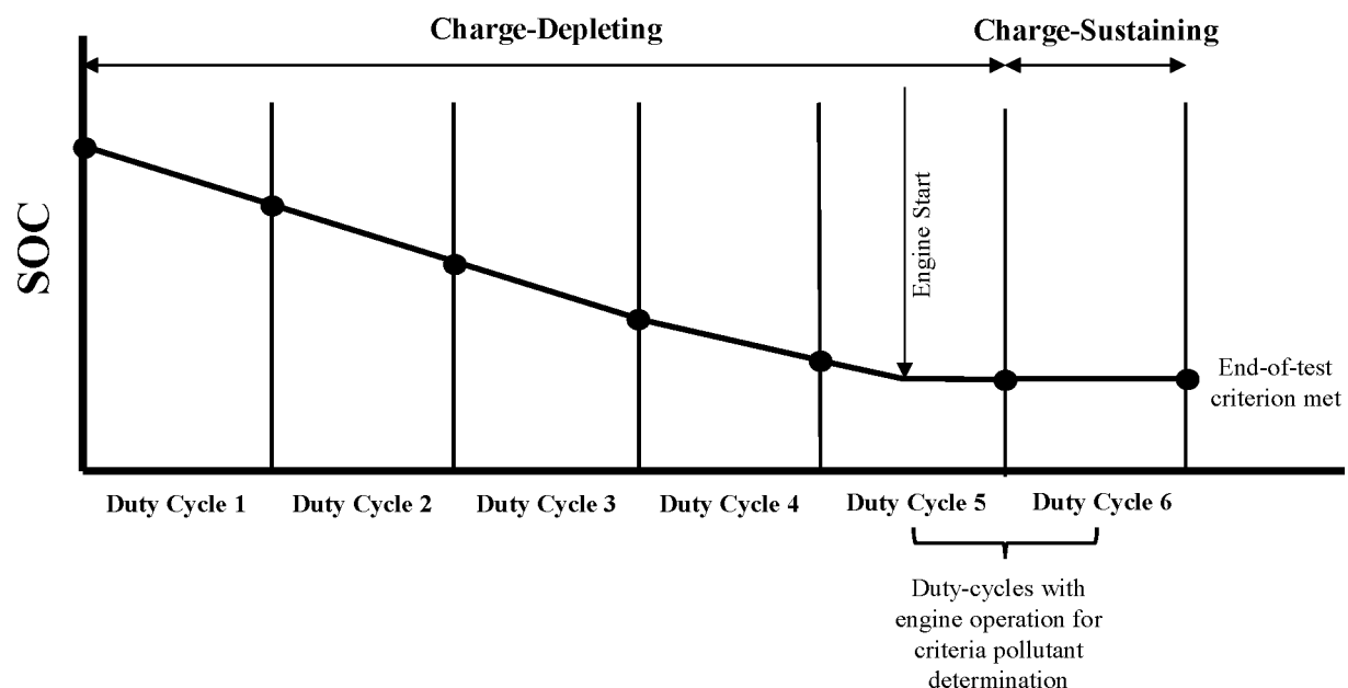
Figure 2 to Paragraph (j)(4) of § 1036.545—Generic Duty-Cycle Charge-Depleting Test Sequence
